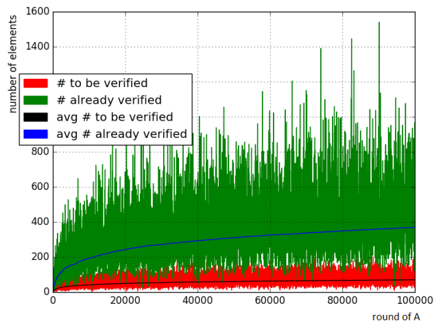
Figure 1: Sum building - first 10^5 rounds of A
